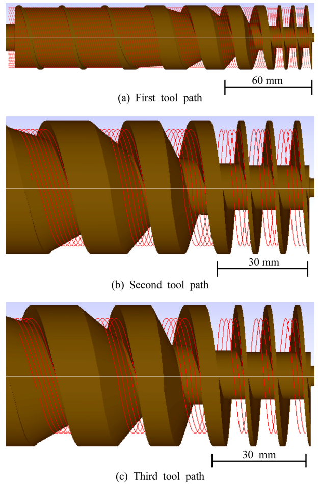
Fig. 10 Tool path modification
