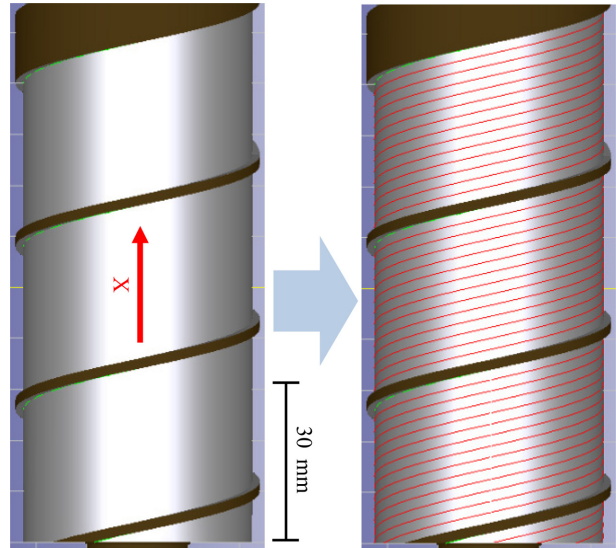
Fig. 7 Tool paths generated by new module
