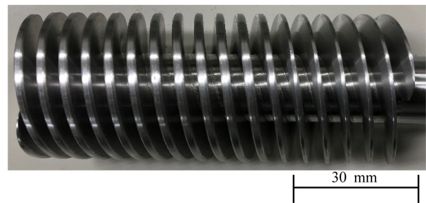
Fig. 1 Example of variable pitch screw (1)
