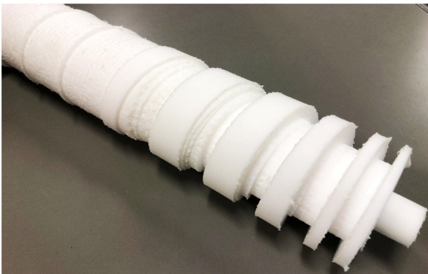
Fig. 13 The result of machining experiment
