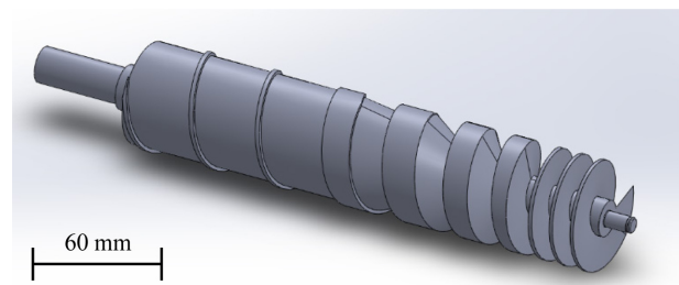
Fig. 3 CAD model of variable pitch screw
