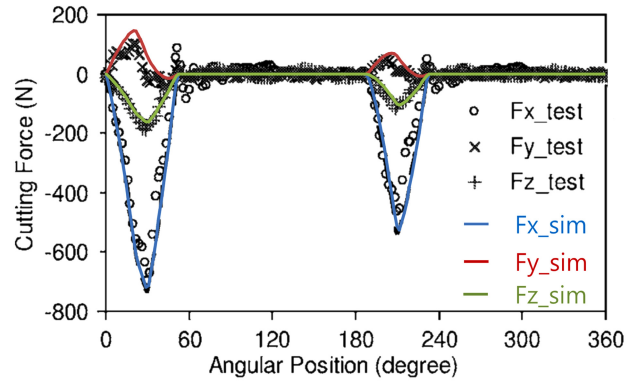
Fig. 1 Cutting force model validation
