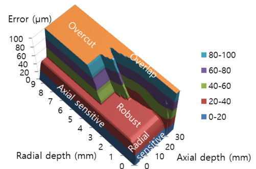
(c) Maximum error of up milling
