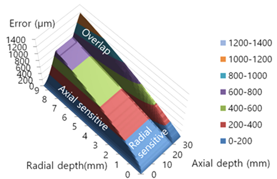
(a) Maximum error of down milling
