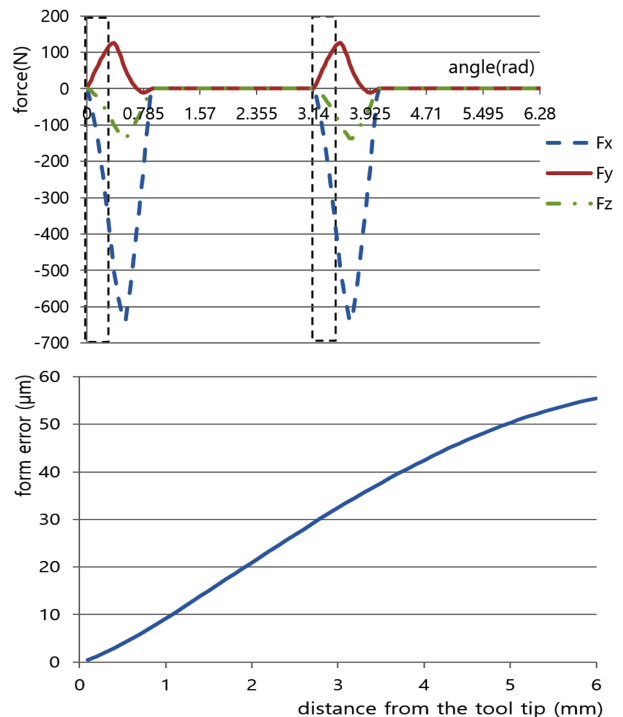
(c) Up milling axial depth 6.1 mm
