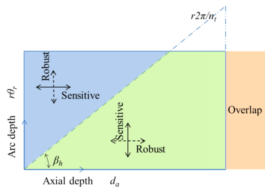
(b) Property zone of down milling
