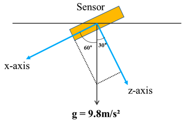
Fig. 1 Principle of accelerometer
