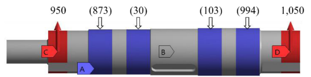
(a) Loading conditions and reaction forces indicated in parentheses at four boundaries [kN]
