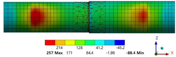
Fig. 7 Maximum principal stress distribution for an asymmetric simple model under symmetric bearing loading (EFS = 500 N/mm 3 ). The left diameter is 190 mm and the right diameter is 200 mm
