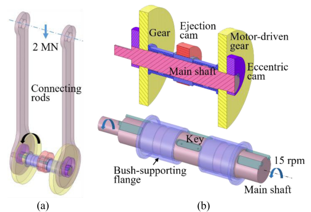
Fig. 1 Adjoining parts to the main shaft: (a) Power train from motor-driven gear to connecting rods, and (b) Upper: Cross-section of main shaft and related parts, and Lower: Main shaft, three sets of keys, and a set of flanges to hold four metal bushes (thrust bearings)
