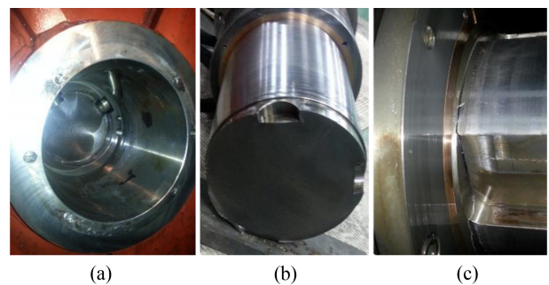
Fig. 4 Failed main shaft: (a) Complete fracture at section A-A in a press, and (b) Failed part taken from (a), (c) crack at section B-B
