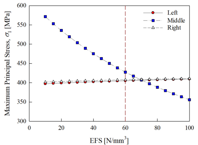
Fig. 11 Maximum principal stresses of the three vulnerable portions of the main shaft as a function of EFS
