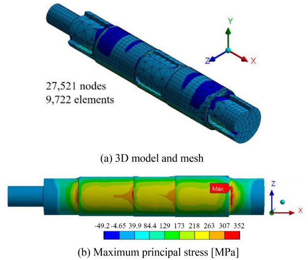
Fig. 13 Structural analysis for the second modified main shaft
