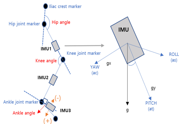
Fig. 5 Definition of lower-limb joint angle
