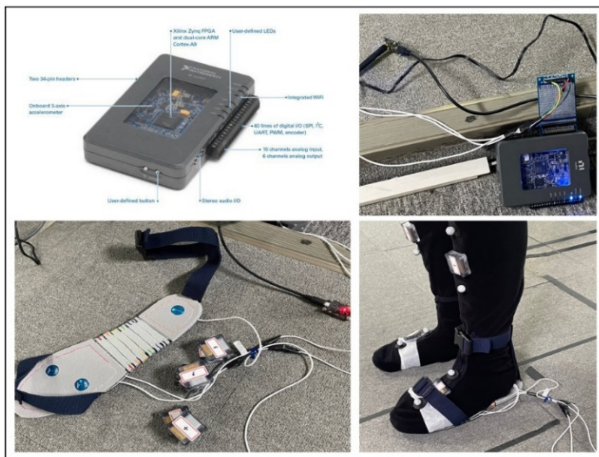
Fig. 3 Data acquisition system by NI myRIO box
