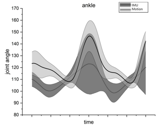
(c) Ankle angle
