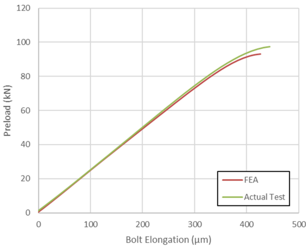
Fig. 7 Cambolt elongation graph
