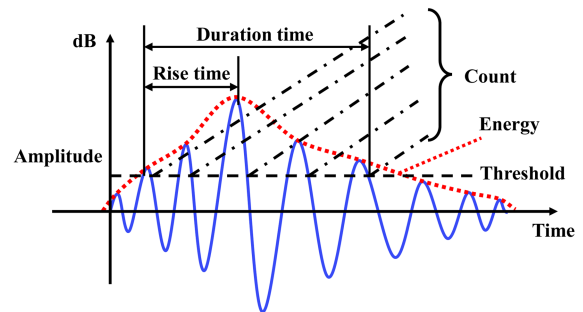
Fig. 2 Schematic figure showing the main AE parameters
