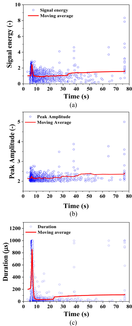
Fig. 5 AE parameters according to time of Case 1: (a) Signal Energy, (b) Peak Amplitude, and (c) Duration
