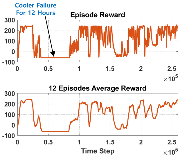
Fig. 7 Episode reward during the training
