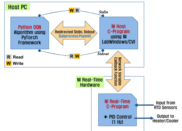
Fig. 6 Data pipeline structure between the Python-code and C-programs
