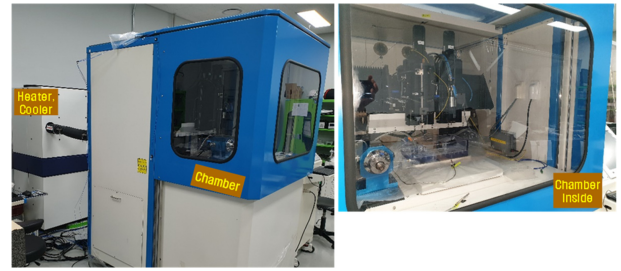
Fig. 3 Experimental chamber for ultra-precision machines
