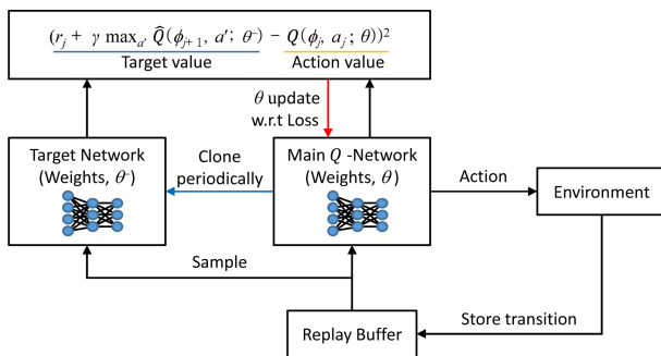
Fig. 2 An illustration of DQN architecture
