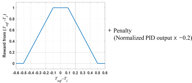
Fig. 4 Computation of reward r_i at each time step
