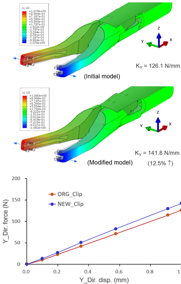
Fig. 6 Lateral stiffness of the initial and modified jaw parts of the blood vessel ligator
