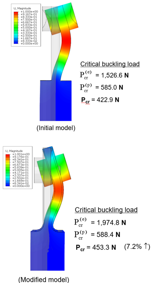
Fig. 9 Critical buckling load of the initial and modified
