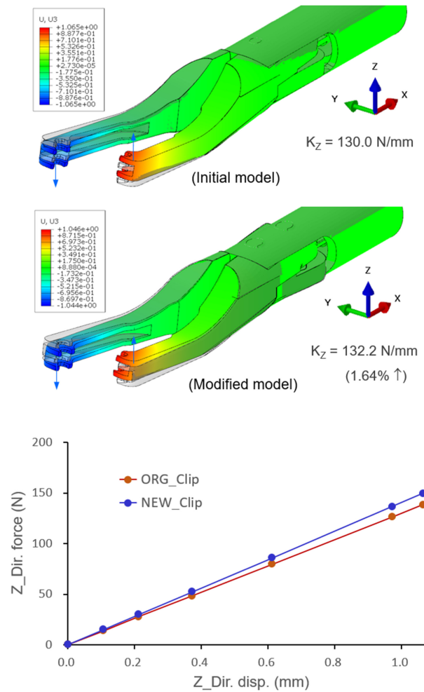
Fig. 7 Twisting stiffness of the initial and modified jaw parts of the blood vessel ligator
