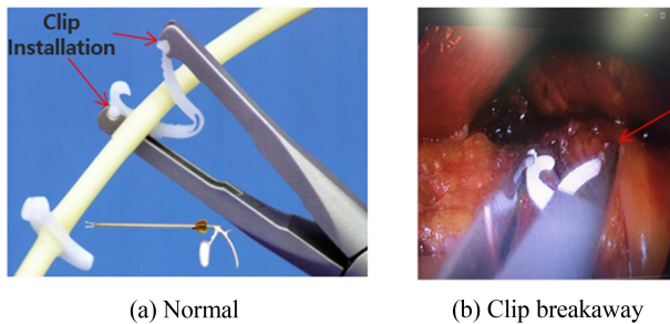
Fig. 2 Normal ligation and clip breakaway due to the excessive clip opening
