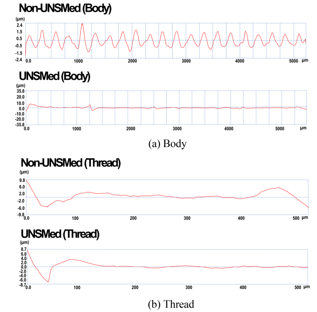
Fig. 8 Surface profiles of the fabricated product with and without UNSM treatment before screw rolling
