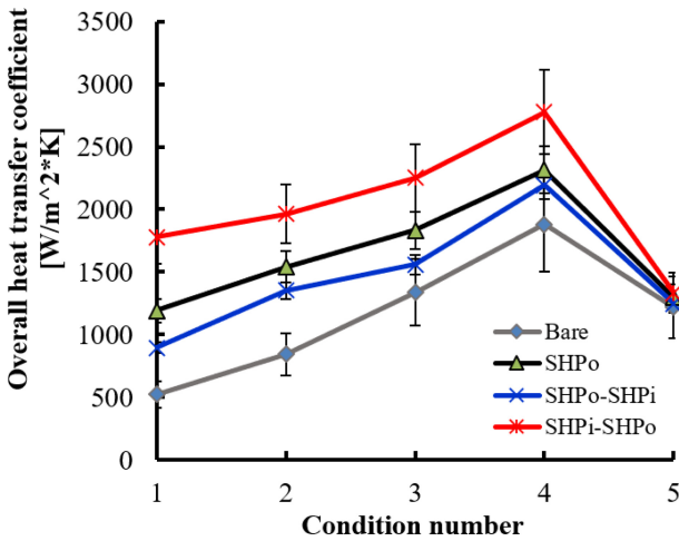
Fig. 6 Evaluation of condensation heat transfer performance of bare, superhydrophobic and hybrid tubes
