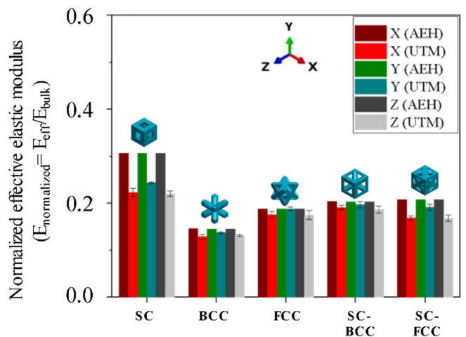
Fig. 5 Normalized effective elastic modulus results of the different types of unit-cells by AEH method and UTM experiment
