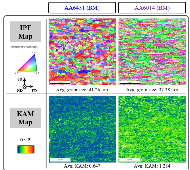
Fig. 12 EBSD results, IPF maps and KAM maps of AA6451 and AA6014
