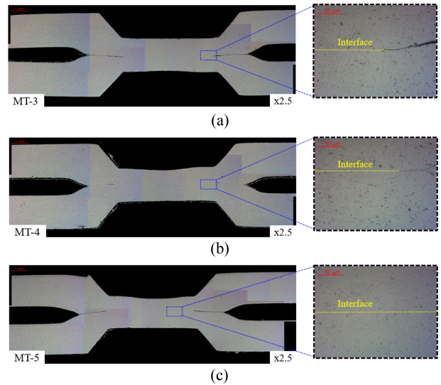
Fig. 11 OM analysis of joint cross section: (a) MT-3, (b) MT-4, (c) MT-5
