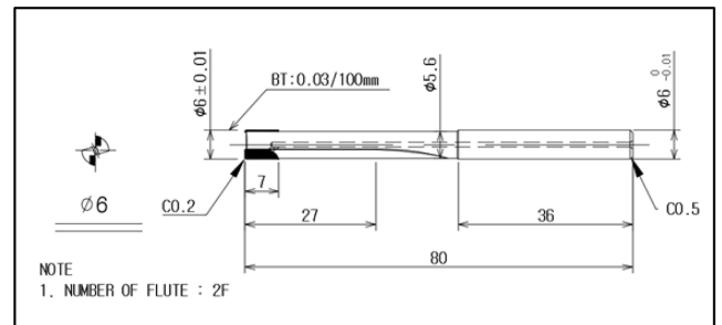
Fig. 8 CAD design and brazing images of PCD tip endmill: (a) 2D CAD of PCD tip endmill and (b) Image of the brazed endmill
