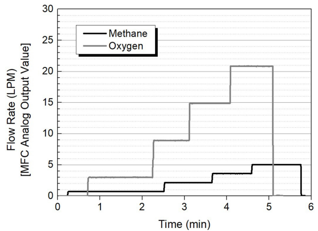
Fig. 9 Variation of MFC output values according to the increase in the MFC scale during flow rate calibration
