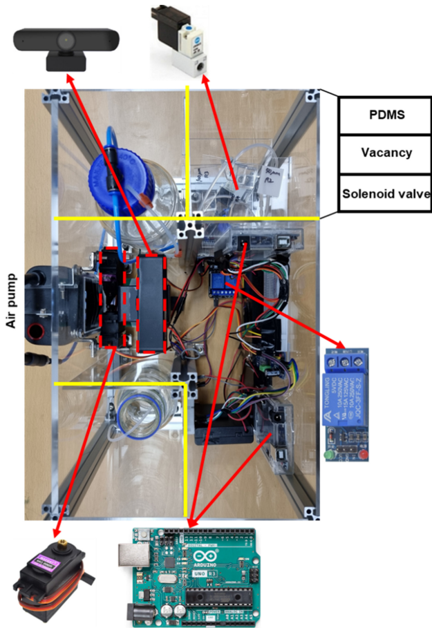
Fig. 1 Appearance of a microfluidic controller utilizing a portable air pump
