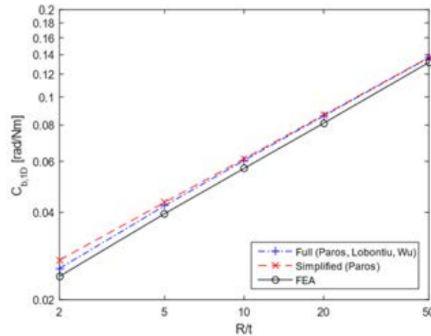
(b) Rotational compliance
