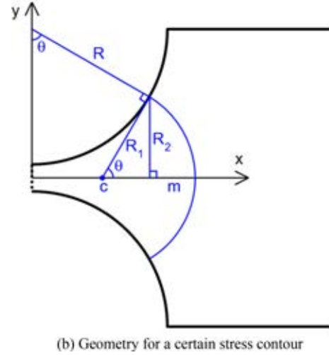
Fig. 7 Stress contour and geometry
