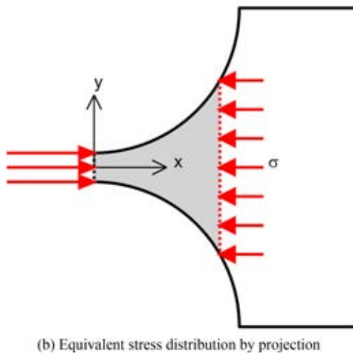
Fig. 6 Free body diagram at a certain stress contour
