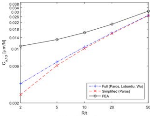
(a) Axial compliance
