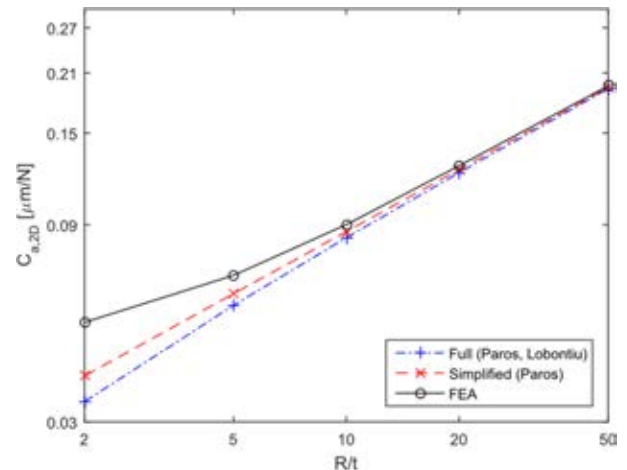
(a) Axial compliance
