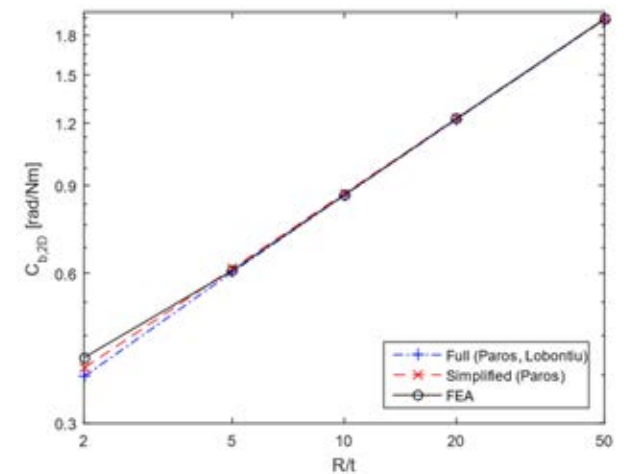
(b) Rotational compliance
