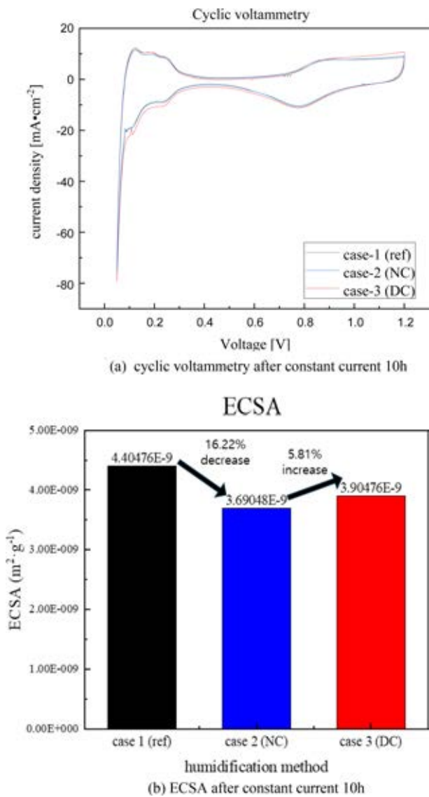
Fig. 4 Cyclic voltammetry after constant current 10h and ECSA
