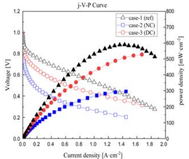
(b) j-V-P curves as initial performance after activation
